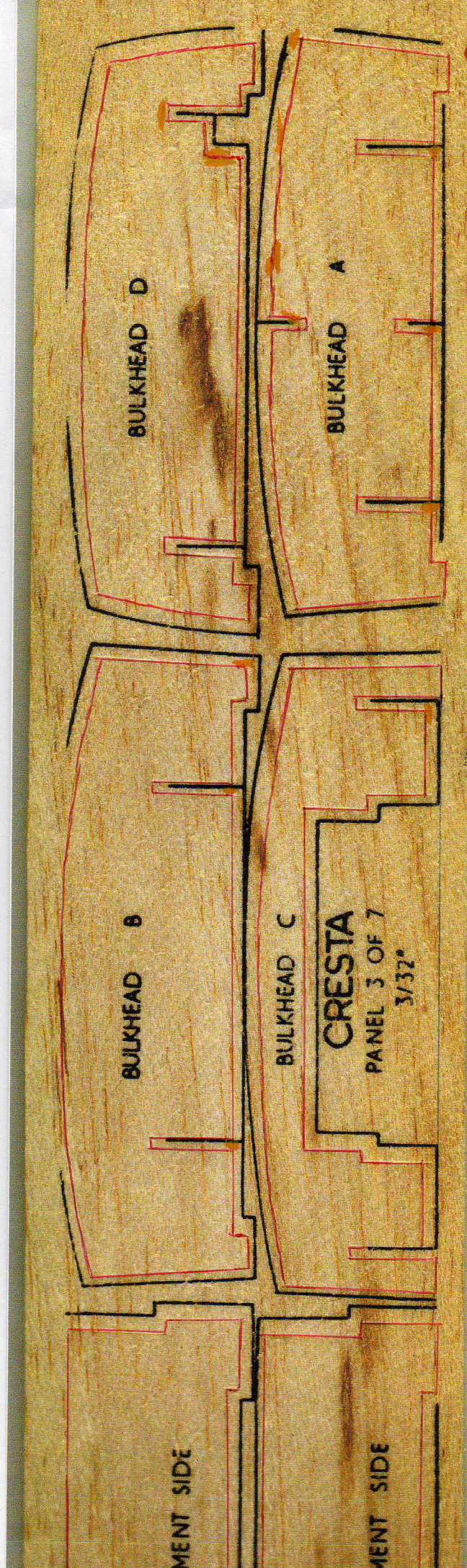
Cresta – Sheet 3. 3.2in x 14.5 in x 3/32“ balsa. One off.
